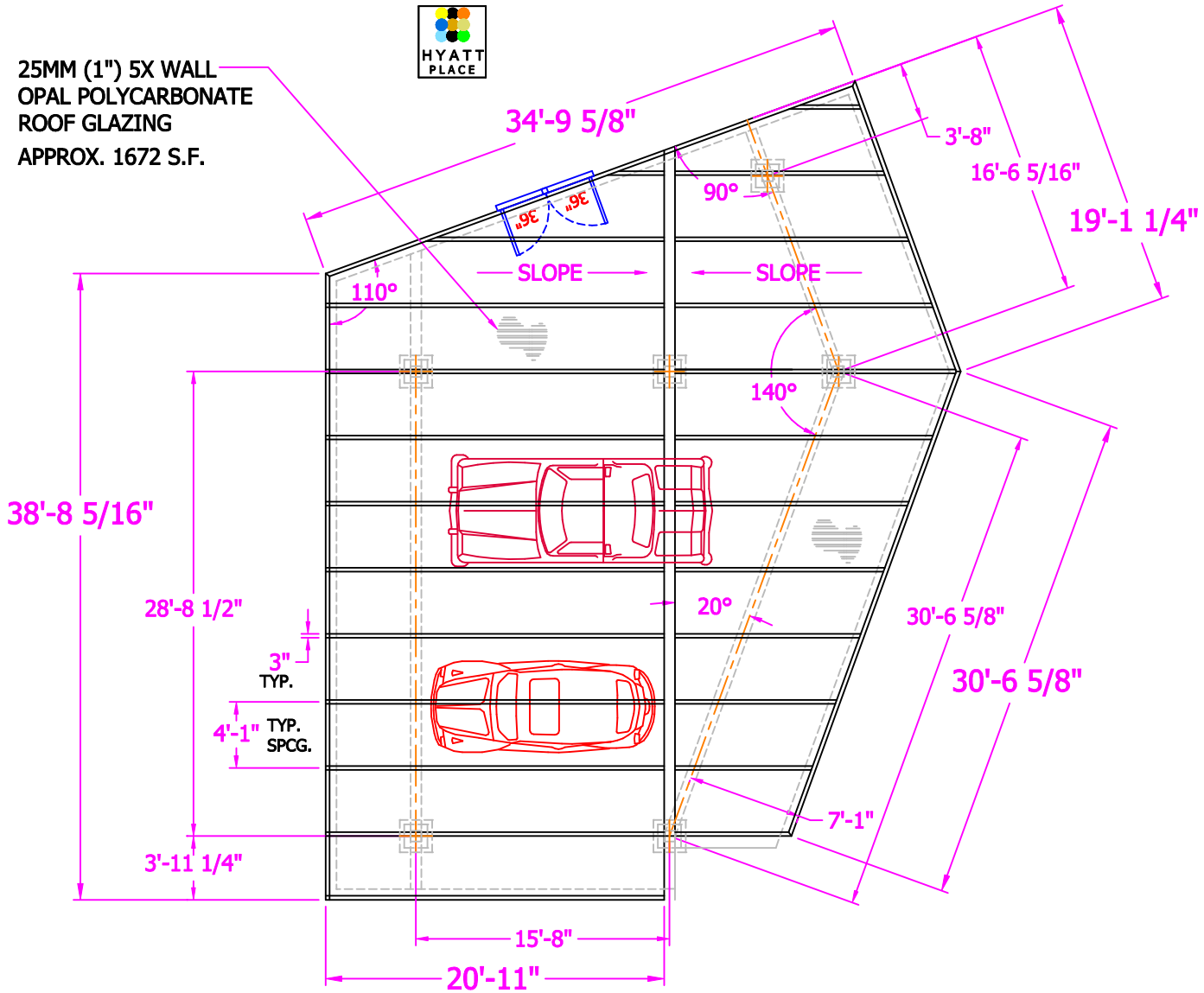
ROOF PLAN
