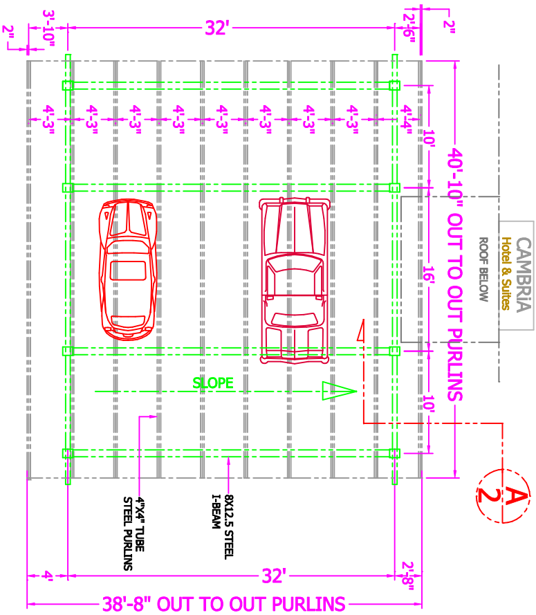
ROOF STEEL PLAN
