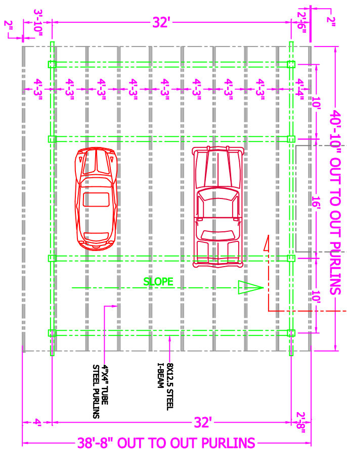
ROOF STEEL PLAN
