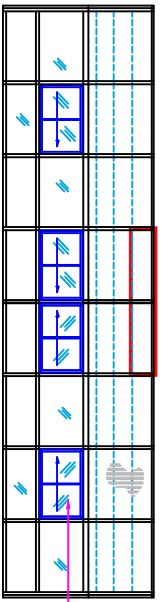
OPPOSITE SIDEWALL ELEV.
