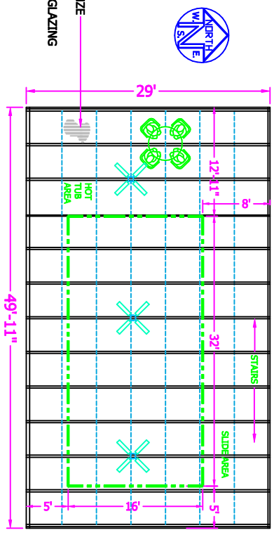
ROOF PLAN
